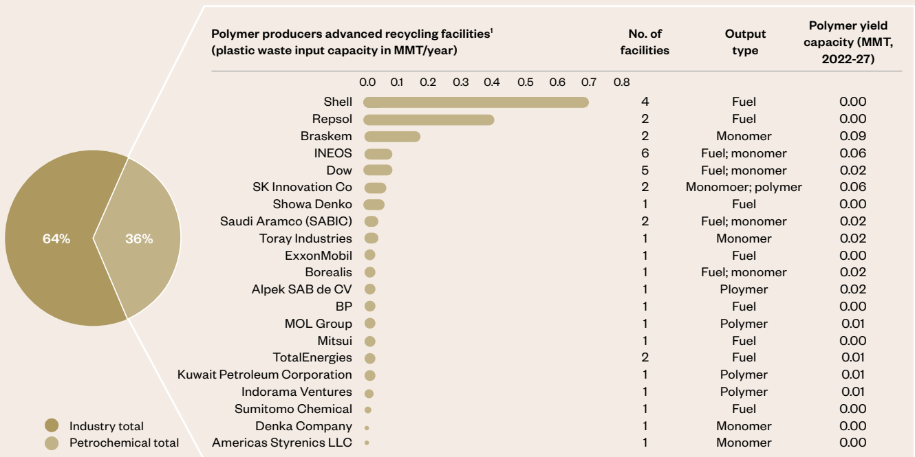
Figure 13: Petrochemical companies expected to develop 2 MMT of chemical recycling capacity by 2027 – but of this expected recycled plastic polymer yield only 0.4 MMT
