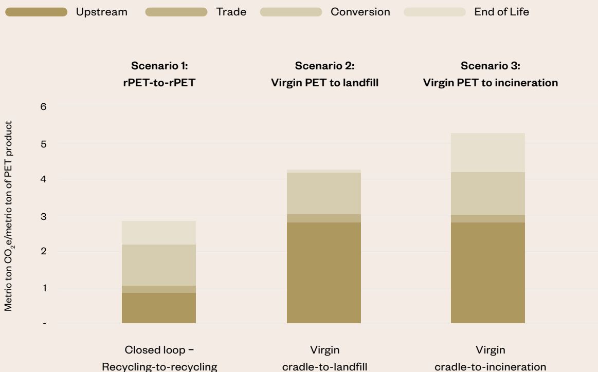
Figure 9: Comparison of cradle-to-grave emissions in a circular versus linear plastics economy
