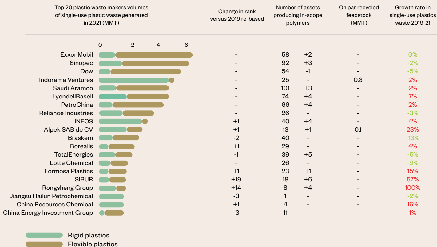
Figure 5: The top 20 list of petrochemical companies producing polymers bound for single-use plastic in 2021 remains effectively unchanged since 2019
