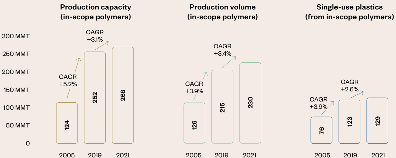
Figure 1: While there is more single-use plastic than ever (+6 MMT 19-21), growth is slower than historical rates and in step with slower polymer capacity expansion
