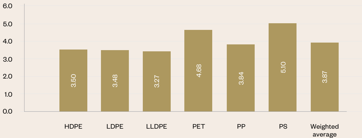
Figure 8: Global variation in cradle-to-grave GHG emissions by polymer type (metric ton CO 2 e/metric ton polymer)
